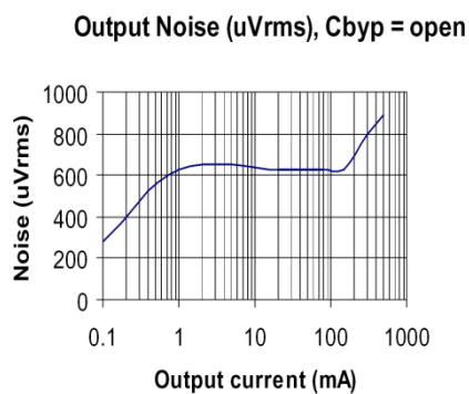
Fig. 20: Output Noise, C_{BYP} = open
